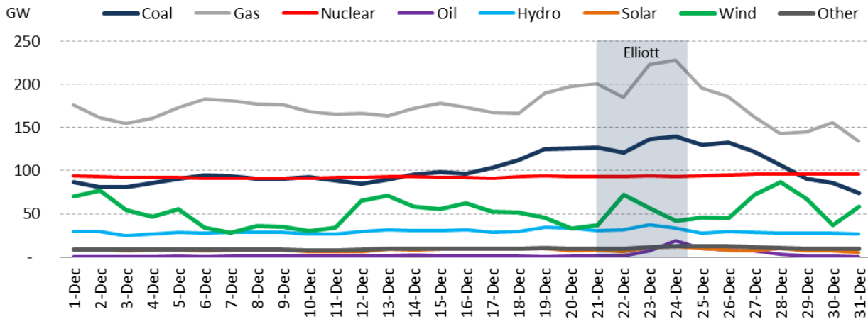
EXHIBIT 4: U.S. LOWER-48 AVERAGE DAILY NET GENERATION BY FUEL TYPE – DECEMBER 2022
